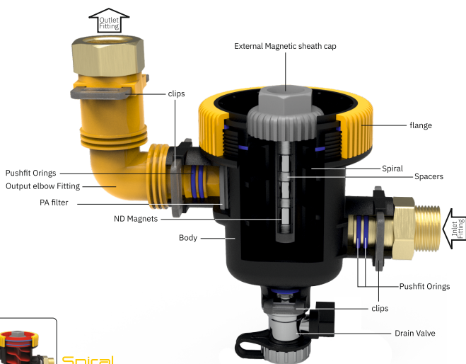
Spiral Conducting WATER FLOW Circulation
