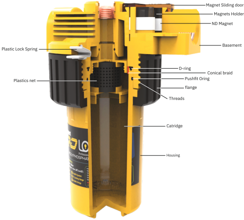
ENHANCED MAGNETS Placement Design
